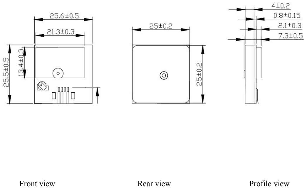
Figure 2: Top view Dimensions
