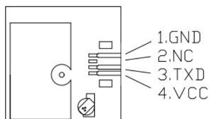
Figure 1: Pin Assignment
