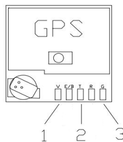
Figure 1: Pin Assignment
