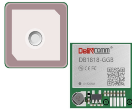
Figure: DB1818-GGB Top View
