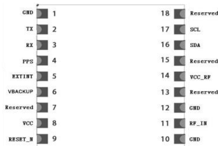
Figure 2: Pin Assignment
