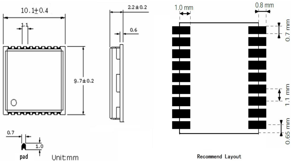
Figure 6: Top view Dimensions
