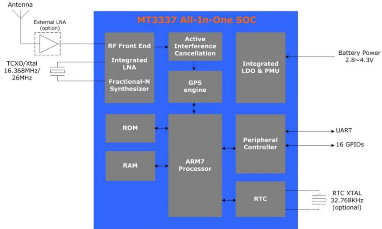
Figure 1: Block Diagram
