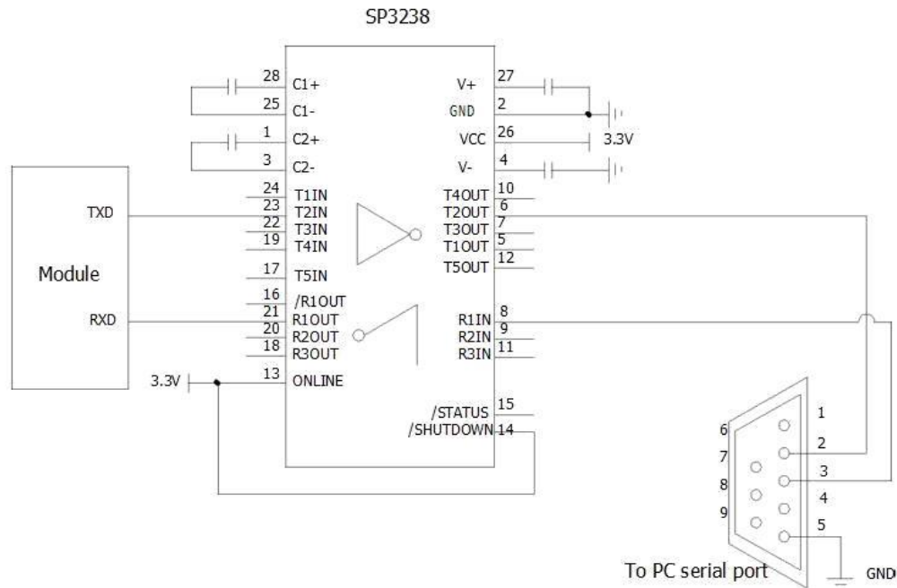
Figure 12: RS-232 Level Shift Circuit
