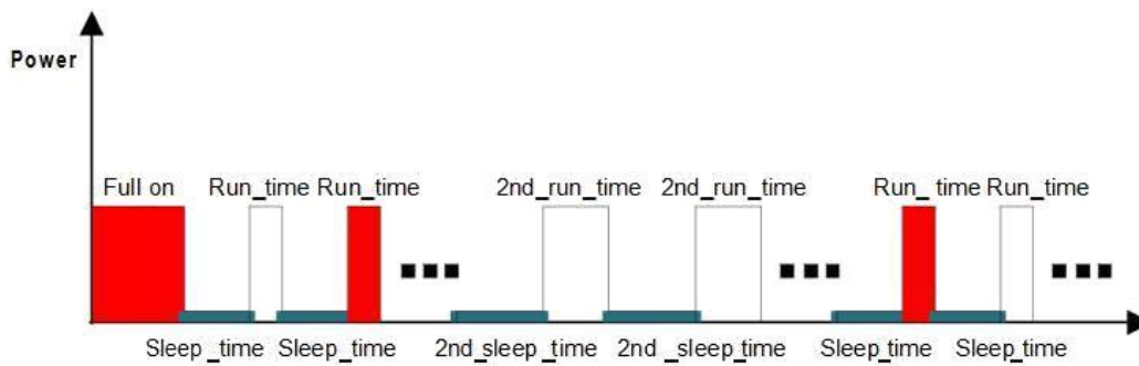
Figure 9: Periodic Mode
